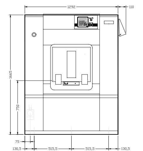
front view HM 330
