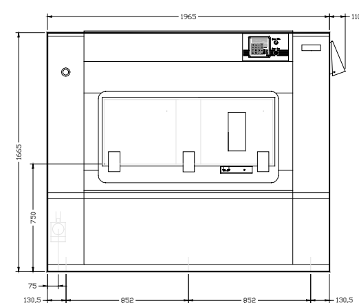
front view HM 670
