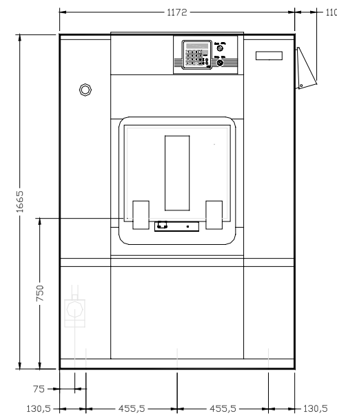
front view HM 270
