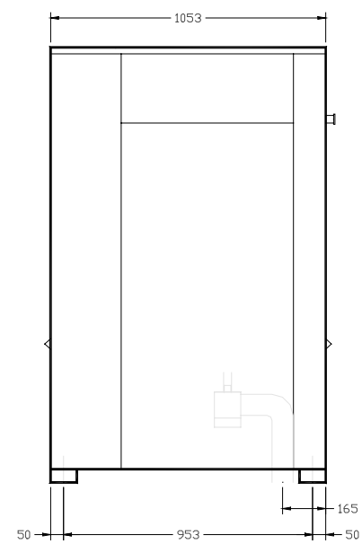
side view HM 270
