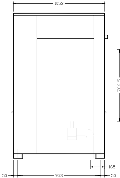
side view HM 330
