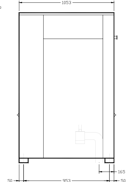
side view HM 670
